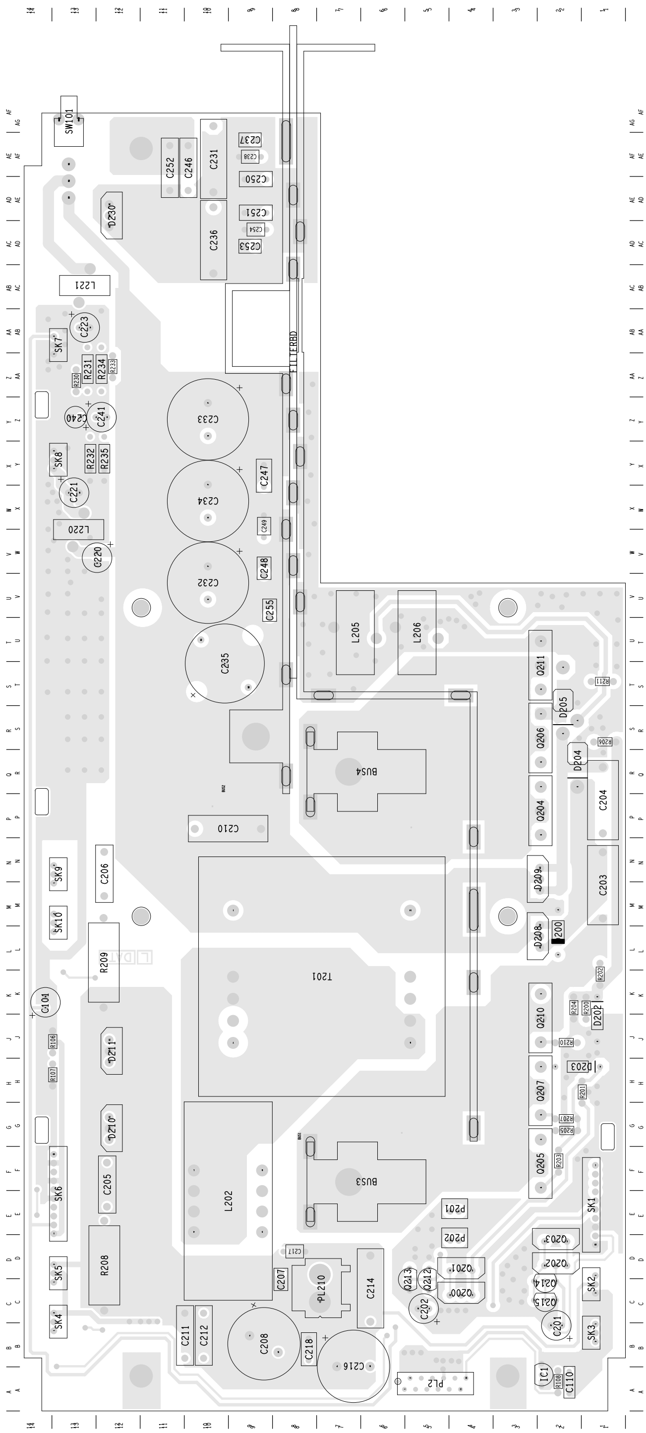
TAIT ELECTRONICS 220-02012-07 A 3006x05_NIS TB8000 DC-DC CONVERTER LAYOUT-PRIMARY-SIDE
